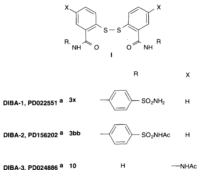
Figure 1. Prototype 2,2'-dithiobisbenzamides.
